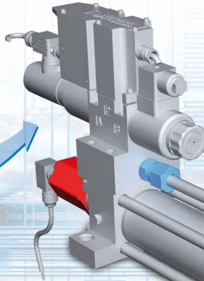
DSE*J proportional valve DXE* servo-proportional valve
